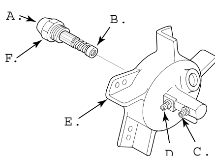
Figur 24 Fjernelse af dysen, 20/29/44 kW Models
