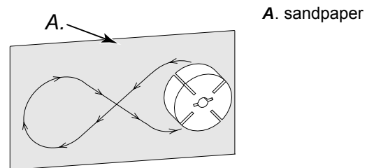
Figure 28 – Sanding rotor.
