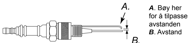
Figur 15 – Tennpluggavstand, 20/29/44 kW modellene
