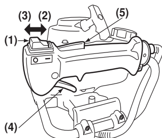
(1) Ontstekingschakelaar (2) RUN (3) STOP (4) Gashendel (5) Gashendelvergendeling
